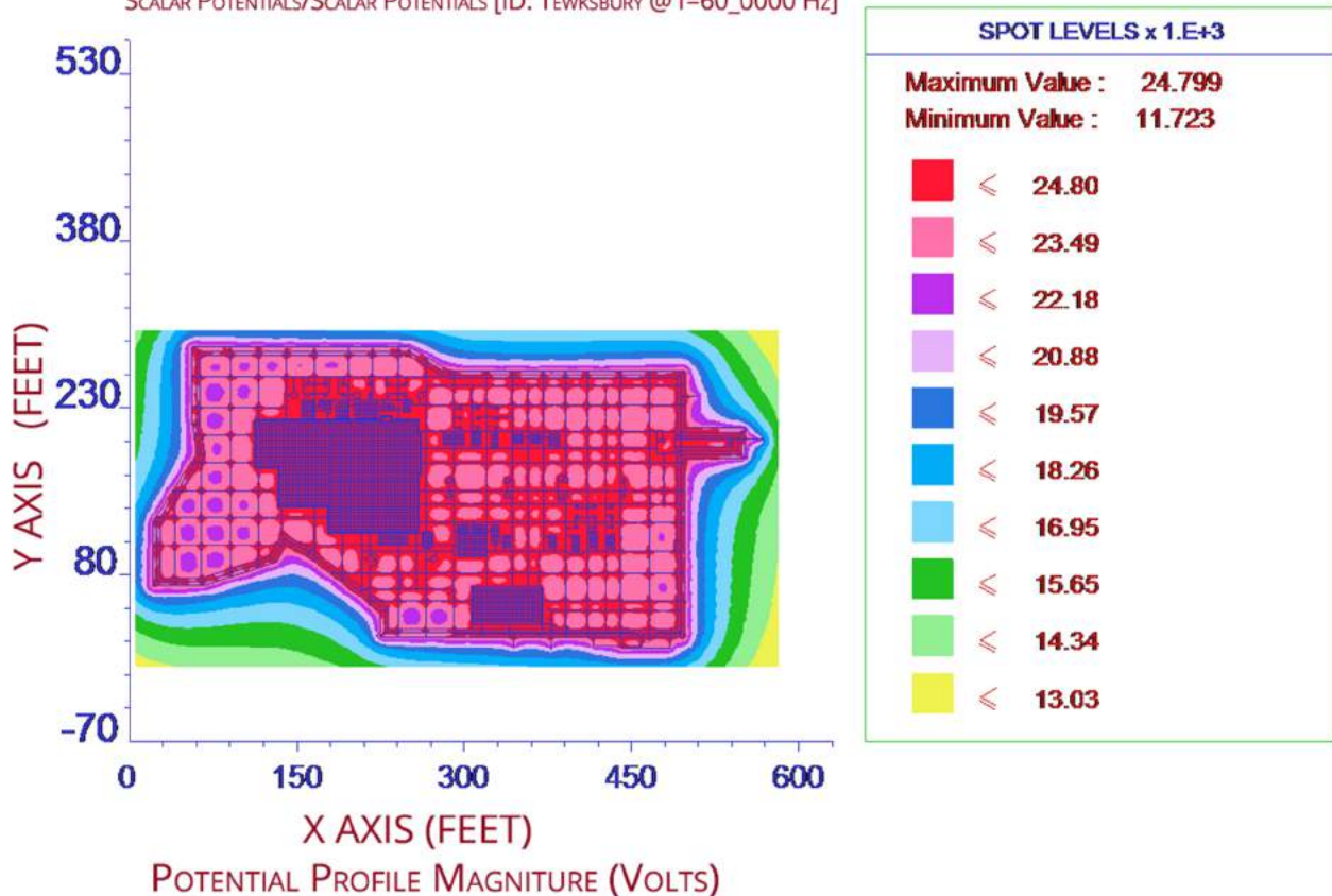
SCALAR POTENTIALS/SCALAR POTENTIALS [ID: TEWKSBURY @ f=60_0000 Hz]
